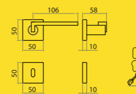
1 Ros 50x50x10 ALL Mont. n°57-58
